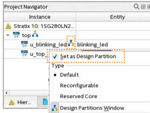
Figure 7. Creating a Design Partition from the Project Hierarchy
